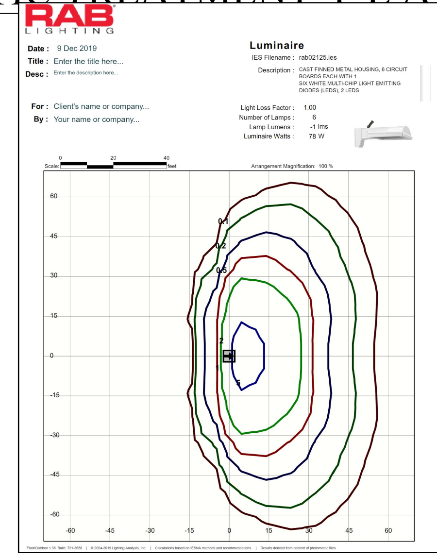
RAB ALED 3T78Y PARKING LOT FIXTURE ON 15' POLE (23-1/2" LONG)
